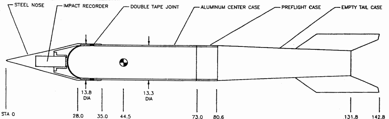
Figure 7. Steel/Aluminum Penetrator Case Illustration
